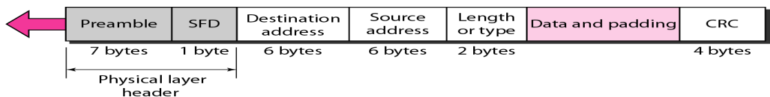
Figure: 802.3 MAC frame
