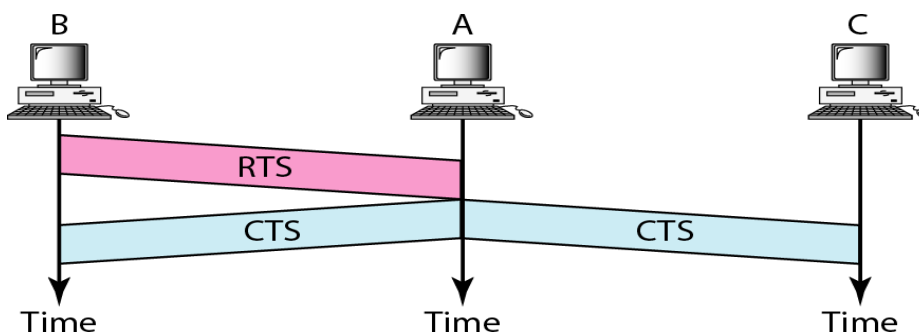
Figure: Use of handshaking to prevent hidden station problem
