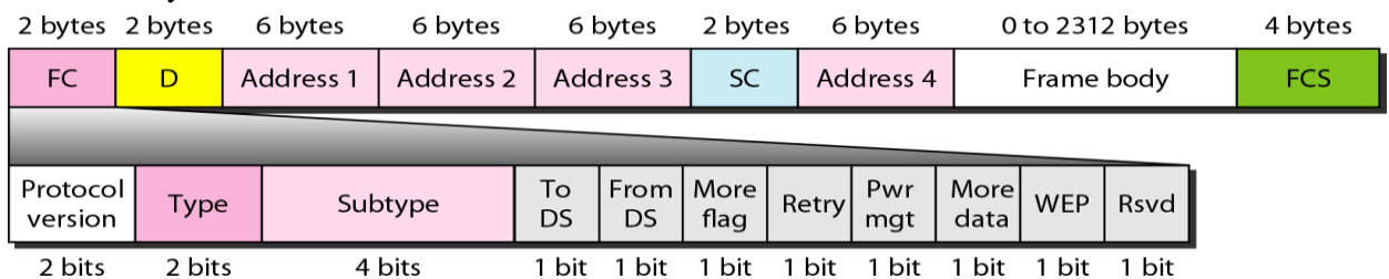
Figure: Frame format
