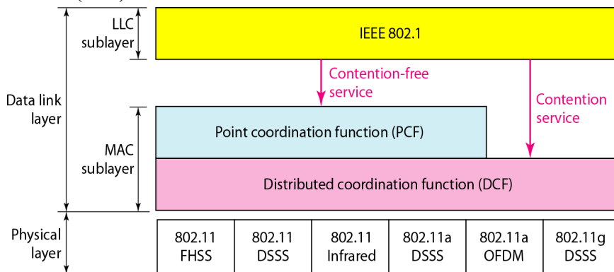
Figure: MAC layers in IEEE 802.11 standard
