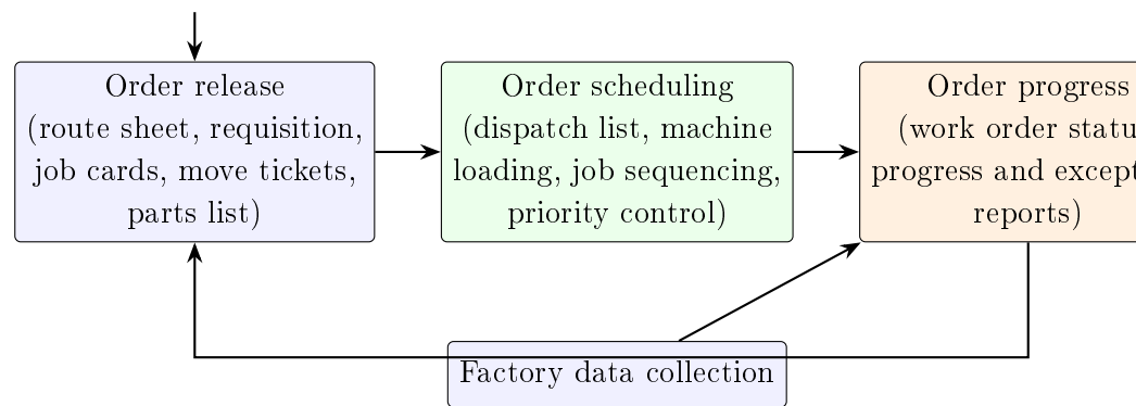
Figure 5.8: Phases in shop floor control
