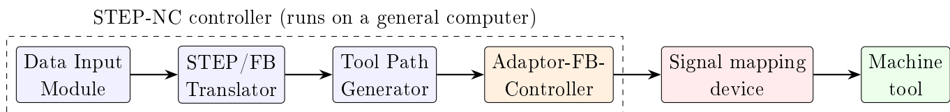
Figure 6.5: Architecture of the feature based STEP-NC controller
