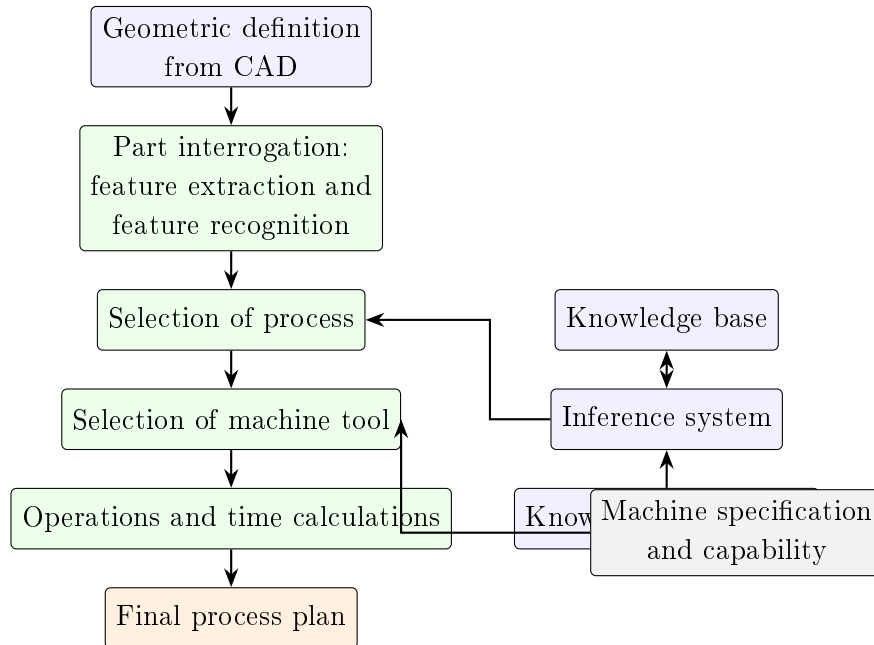
Figure 5.5: Generative process planning
