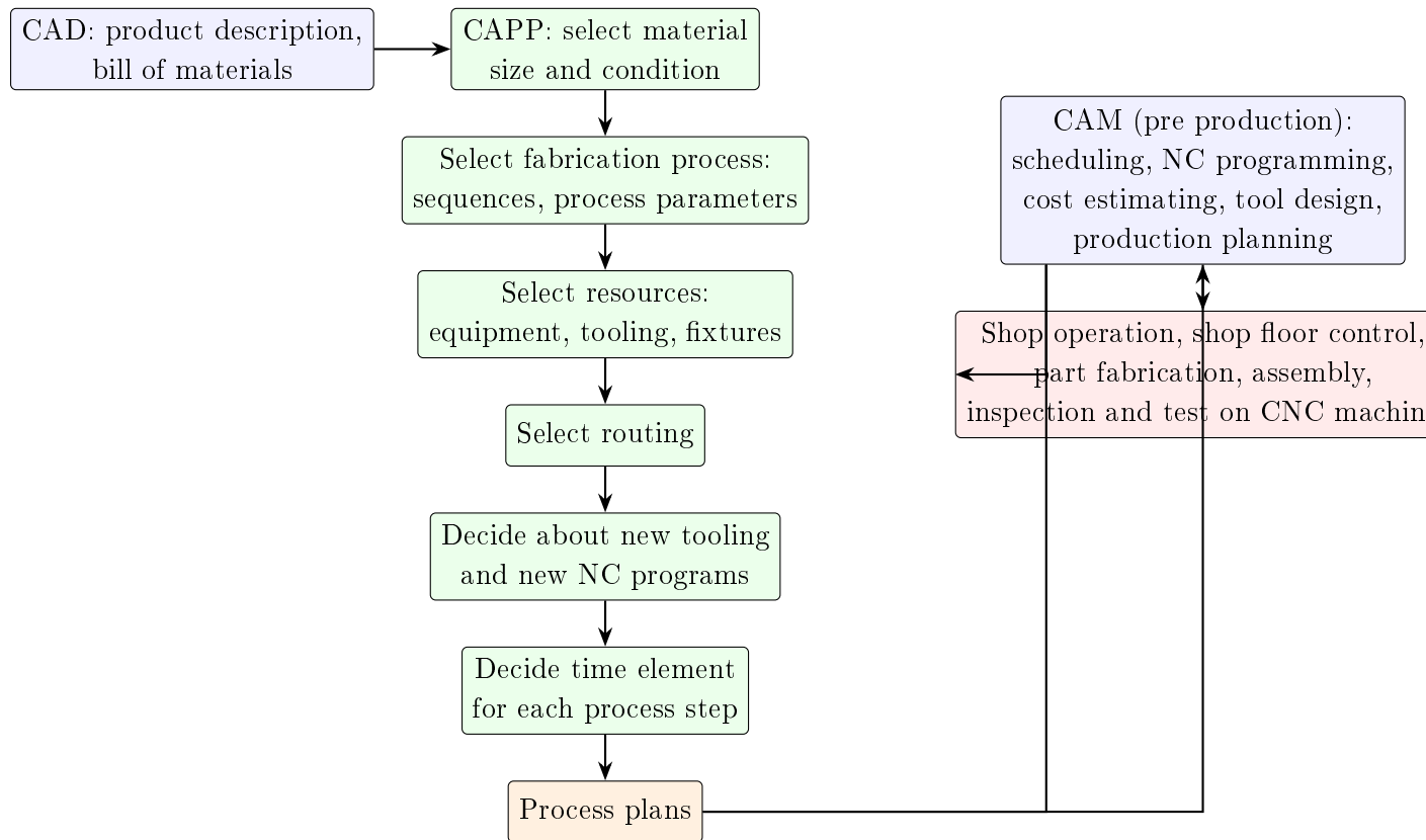
Figure 5.3: Role of CAPP between CAD and CAM
