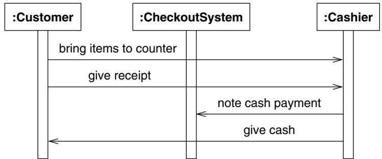
Figure A7.3 Sequence diagram for a return of items
