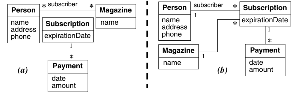
Figure E3.13 Class diagram for magazine subscriptions
