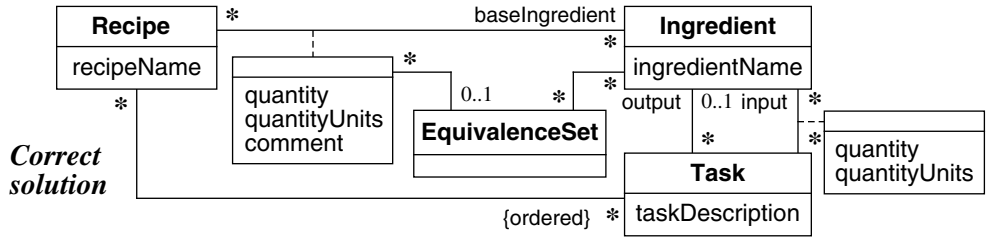
Figure A4.16 Correct class model for recipes with alternate ingredients
