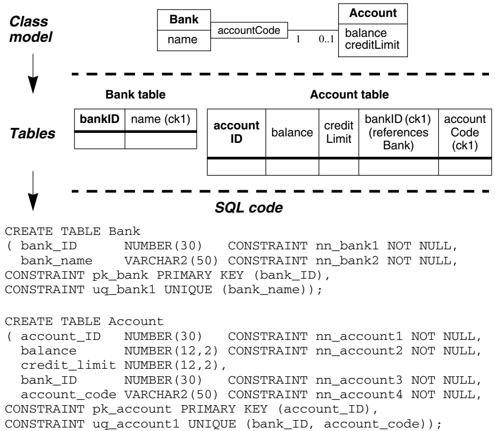
Figure 19.7 Implementing qualified associations. Treat each one like the association without the qualifier.
