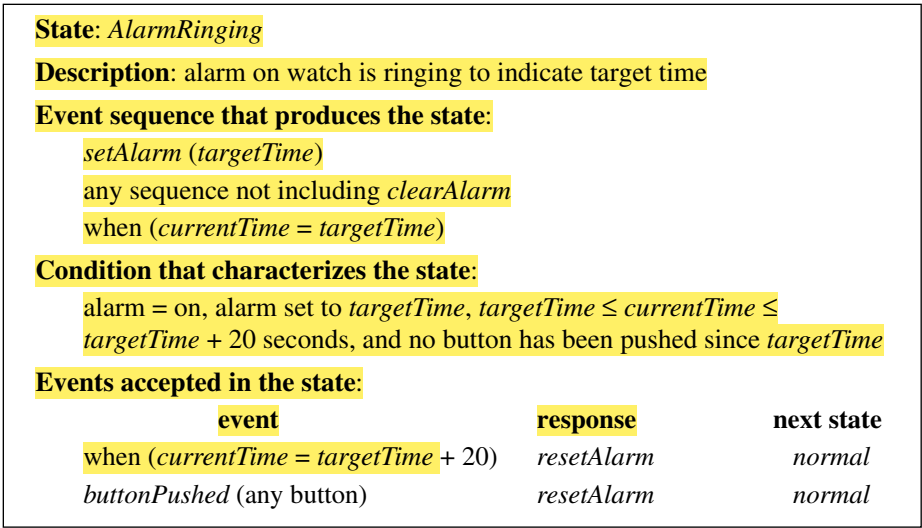
Figure 5.6 Various characterizations of a state. A state specifies the response of an object to input events.
