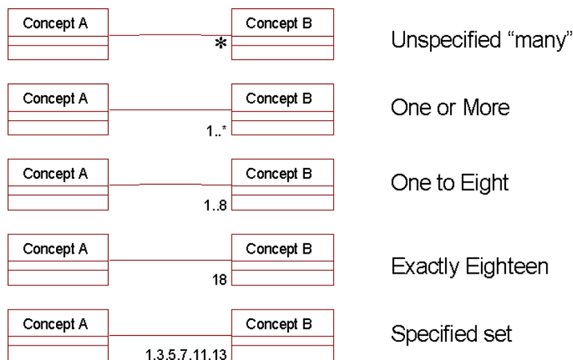
Figure 38 - Example Cardinalities
