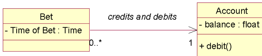
Figure 53 - The Class Diagram, complete!
