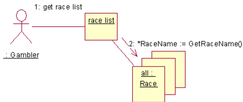
Figure 46 - Collaboration Diagram
