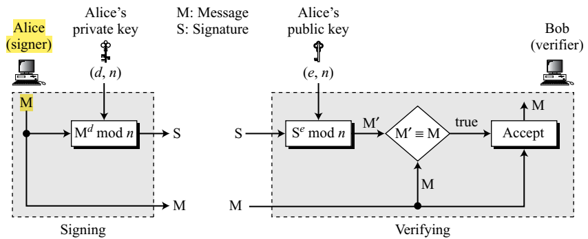
Figure 13.7 RSA digital signature scheme
