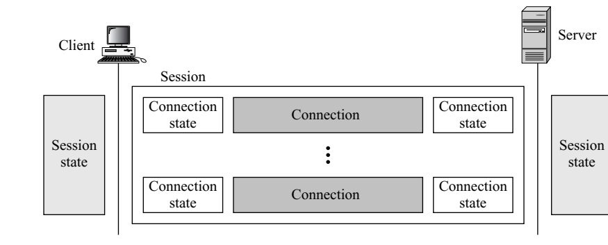
Figure 17.11 A session and connections
