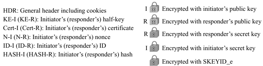
Figure 18.26 Aggressive mode, revised public-key method
