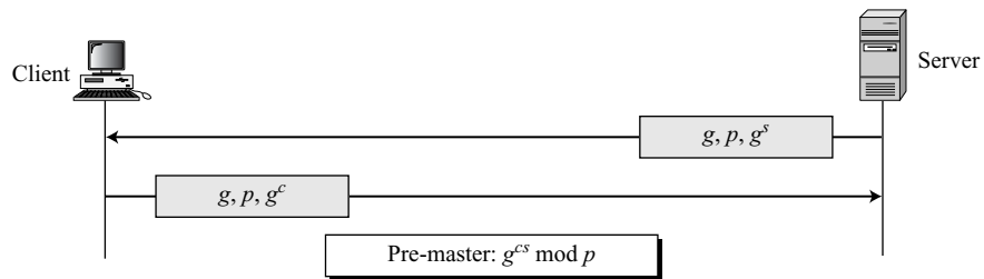
Figure 17.4 Anonymous Diffie-Hellman key exchange
