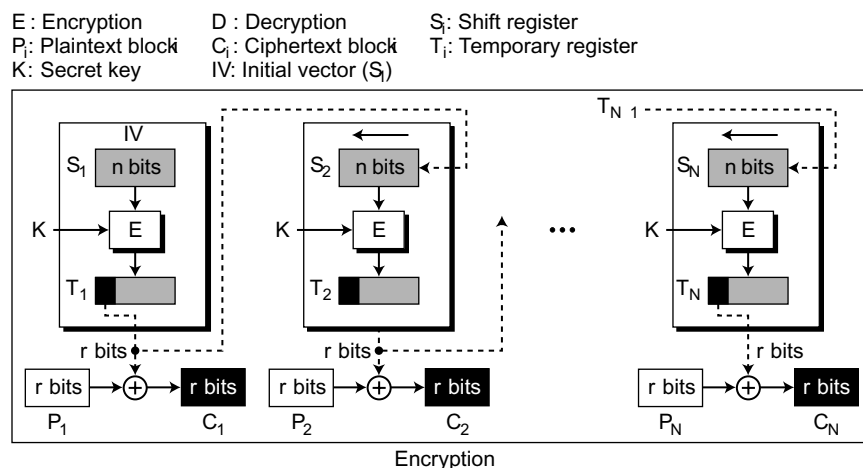
Figure 8.6 Encryption in output feedback (OFB) mode
