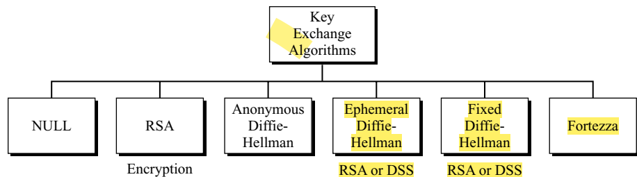
Figure 17.2 Key-exchange methods
