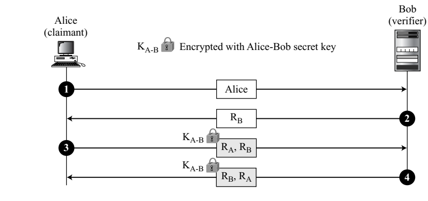
Figure 14.7 Bidirectional authentication
