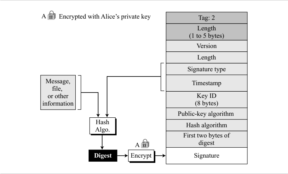
Figure 16.16 Signature packet
