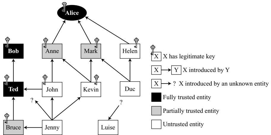
Figure 16.9 Trust model
