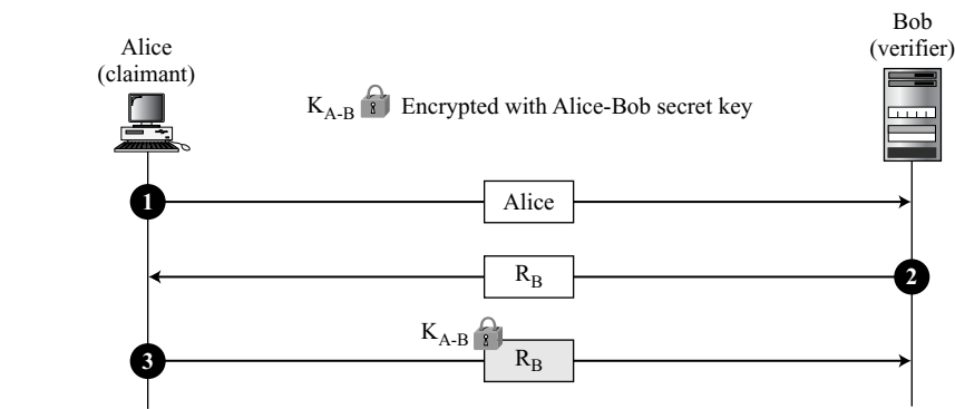
Figure 14.5 Nonce challenge
