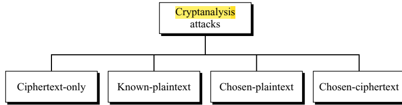
Figure 3.3 Cryptanalysis attacks
