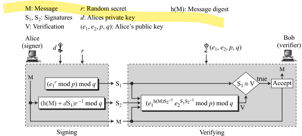
Figure 13.14 DSS scheme
