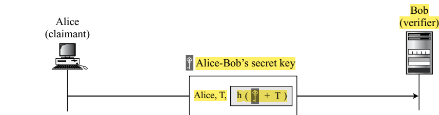
Figure 14.8 Keyed-hash function
