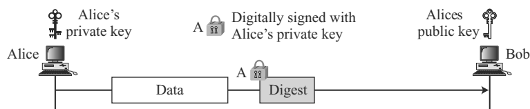
Figure 16.3 An authenticated message
