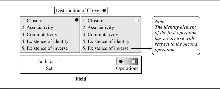
Figure 4.5 Field
