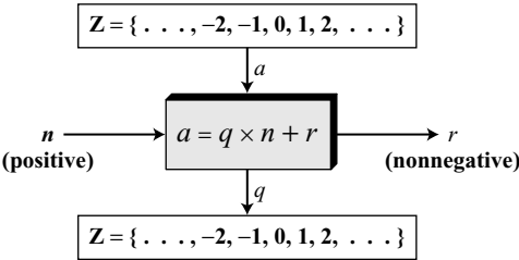
Figure 2.4 Division algorithm for integers
