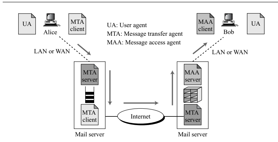
Figure 16.1 E-mail architecture
