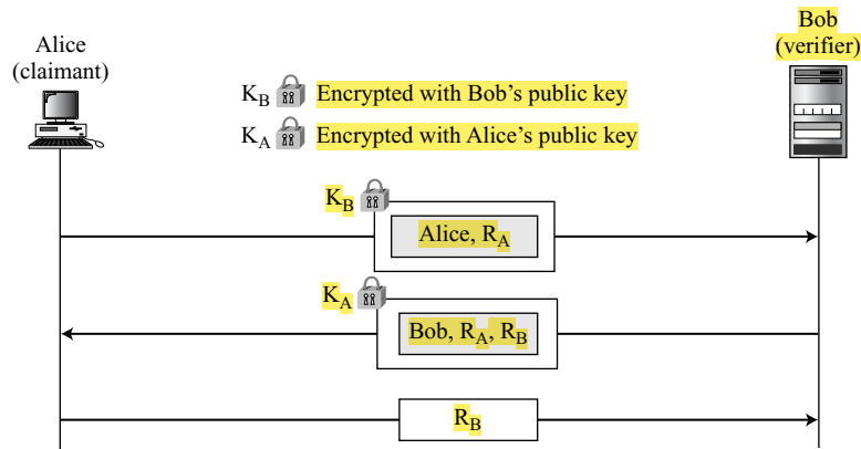
Figure 14.10 Bidirectional, asymmetric-key
