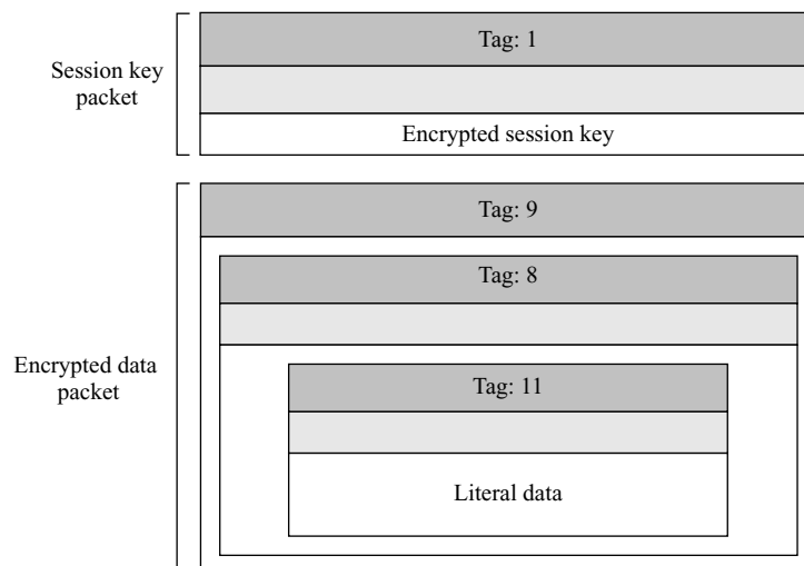
Figure 16.20 Encrypted message
