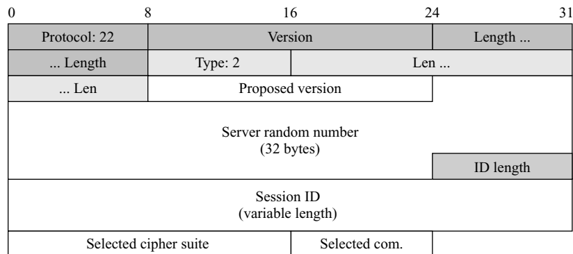
Figure 17.29 ServerHello message
