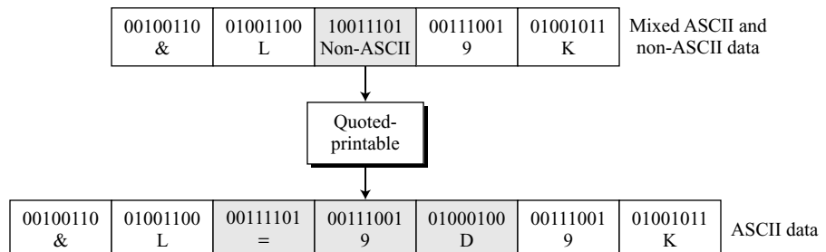
Figure 16.26 Quoted-printable
