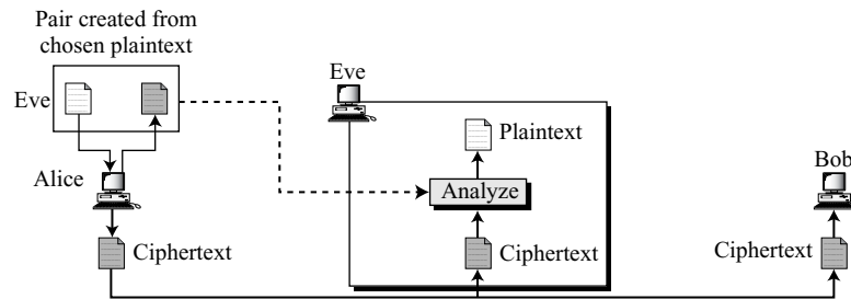
Figure 3.6 Chosen-plaintext attack
