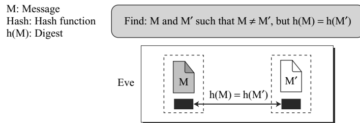
Figure 11.6 Collision
