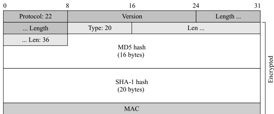
Figure 17.37 Finished message
