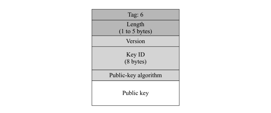
Figure 16.18 Public-key packet
