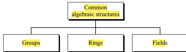
Figure 4.1 Common algebraic structures
