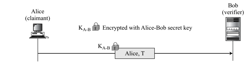
Figure 14.6 Timestamp challenge
