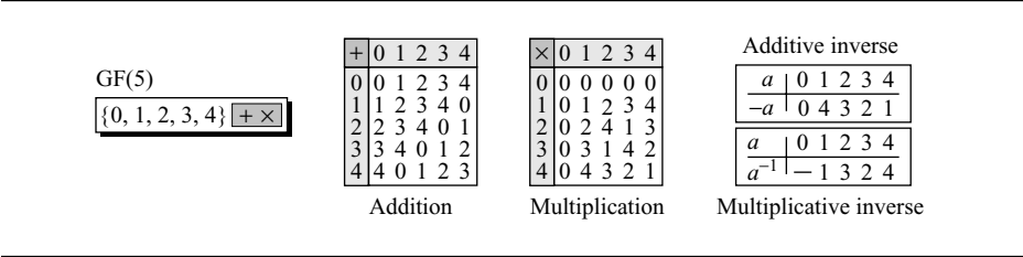
Figure 4.7 GF(5) field
