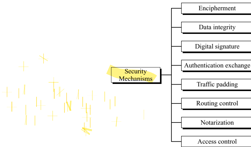
Figure 1.4 Security mechanisms
