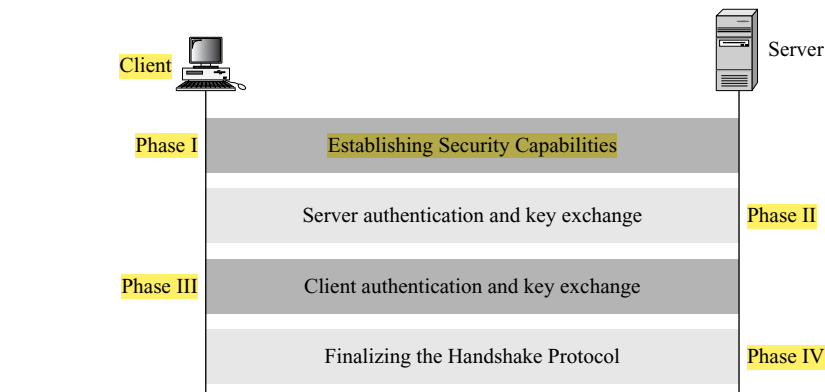
Figure 17.13 Handshake Protocol
