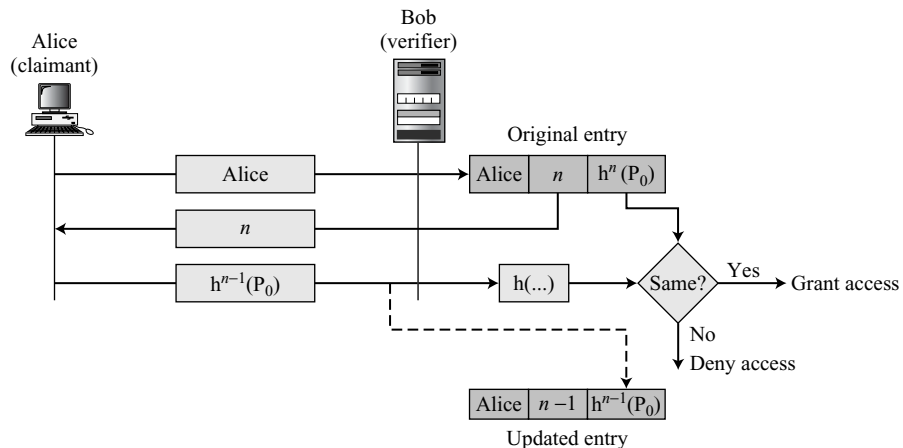
Figure 14.4 Lamport one-time password
