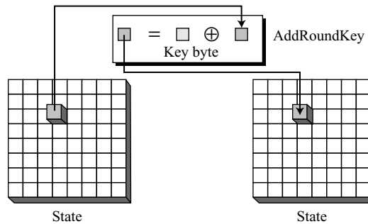
Figure 12.20 AddRoundKey transformation in the Whirlpool cipher
