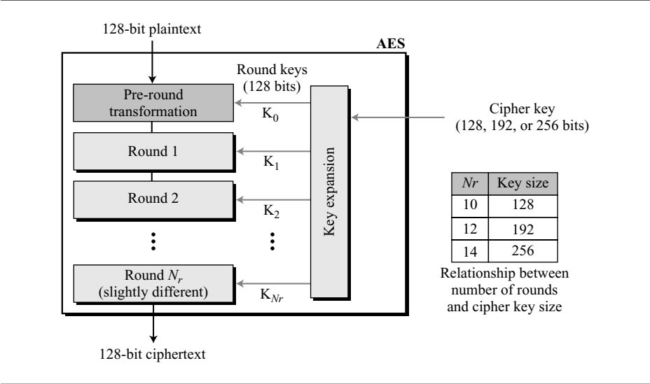
Figure 7.1 General design of AES encryption cipher
