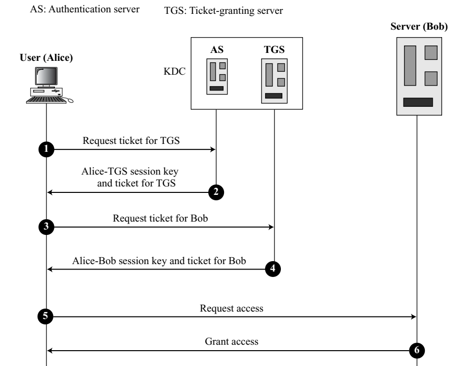
Figure 15.7 Kerberos servers
