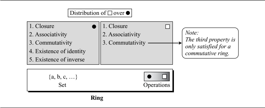
Figure 4.4 Ring
