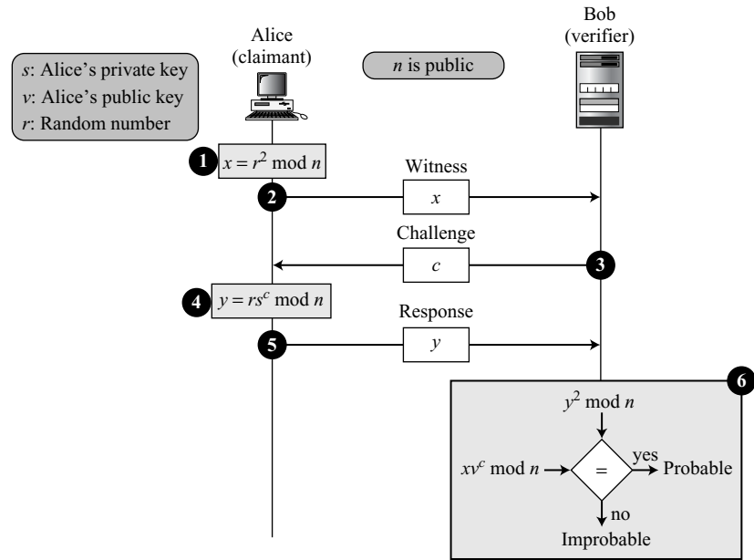
Figure 14.13 Fiat-Shamir protocol
