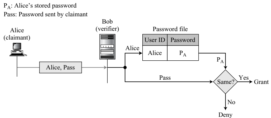
Figure 14.1 User ID and password file
