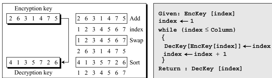
Figure 3.23 Key inversion in a transposition cipher
