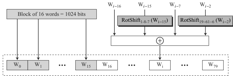
Figure 12.9 Word expansion in SHA-512
