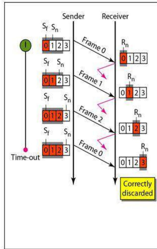
a. Window size < 2^m
