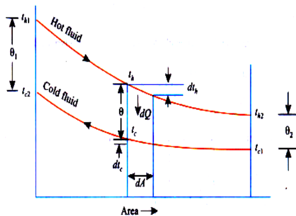
Parallel Flow
